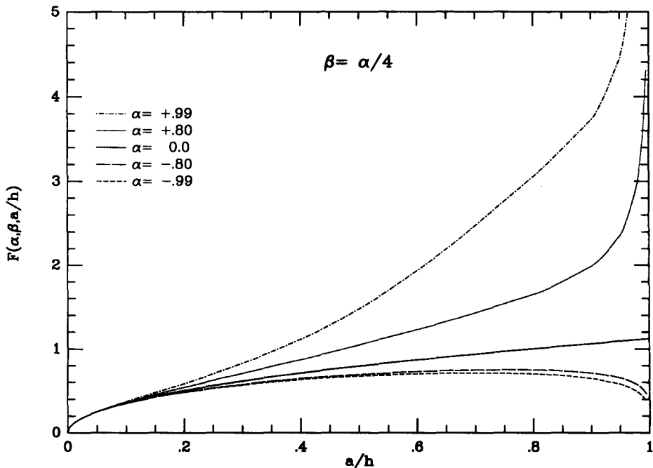
Fig. 8. Plot of F(\alpha, \beta, a/h) vs a/h (partially cracked film problem) for \beta = \alpha/4 .
